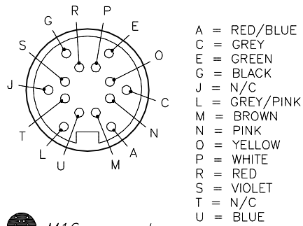
M16 connector
